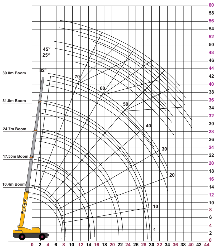
WORKING RANGE - MAIN BOOM
