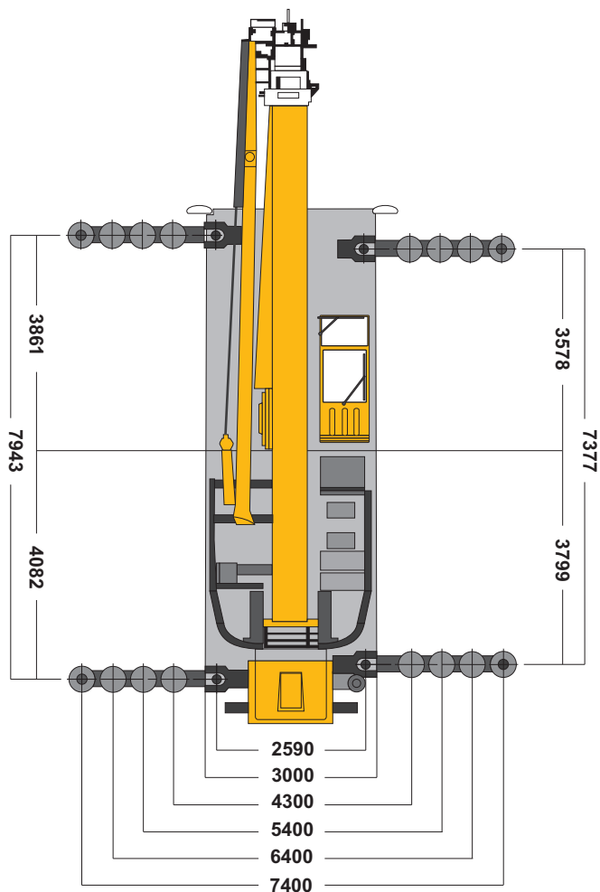
GENERAL DIMENSIONS
