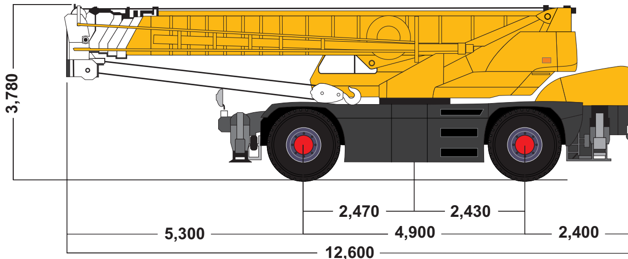
GENERAL DIMENSIONS
